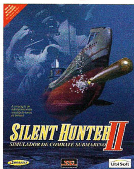
Silent Hunter 2
